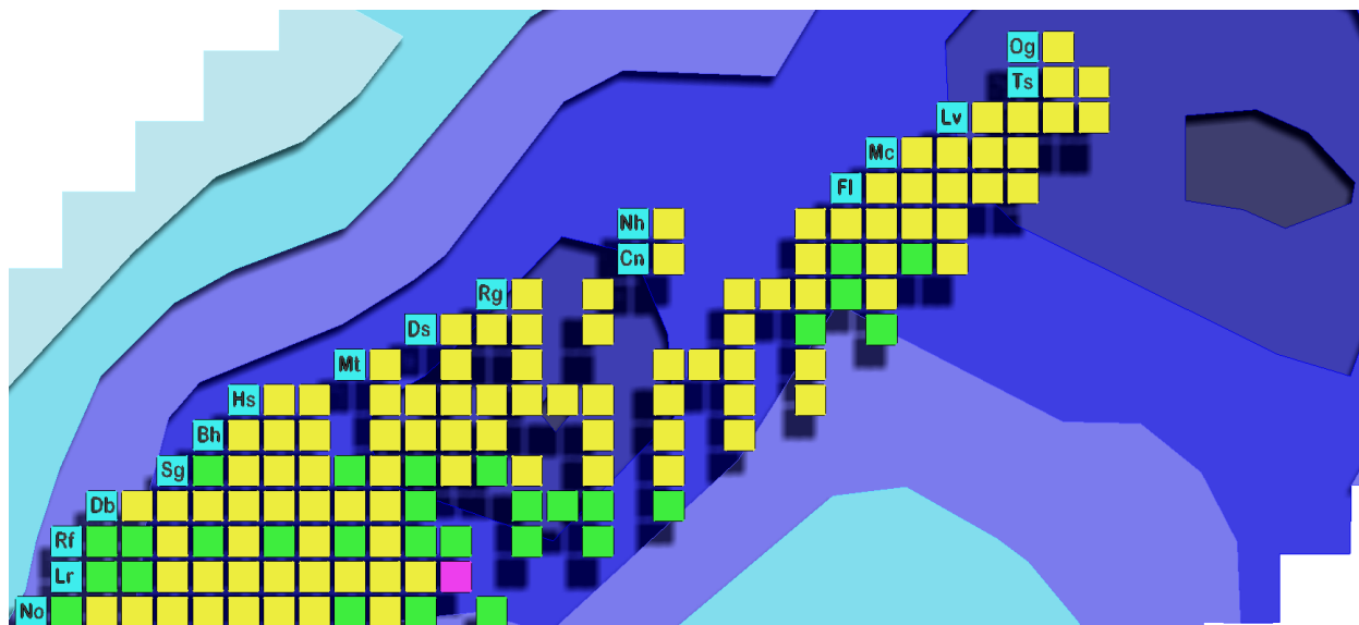
Figure 1.1: Nuclear Chart with the Island of Stability. Known isotopes are shown by their preferred decay mode, either alpha (yellow), beta (magenta) or spontaneous fission (green). These are on a backdrop of predicted shell effects from [Sob01].
