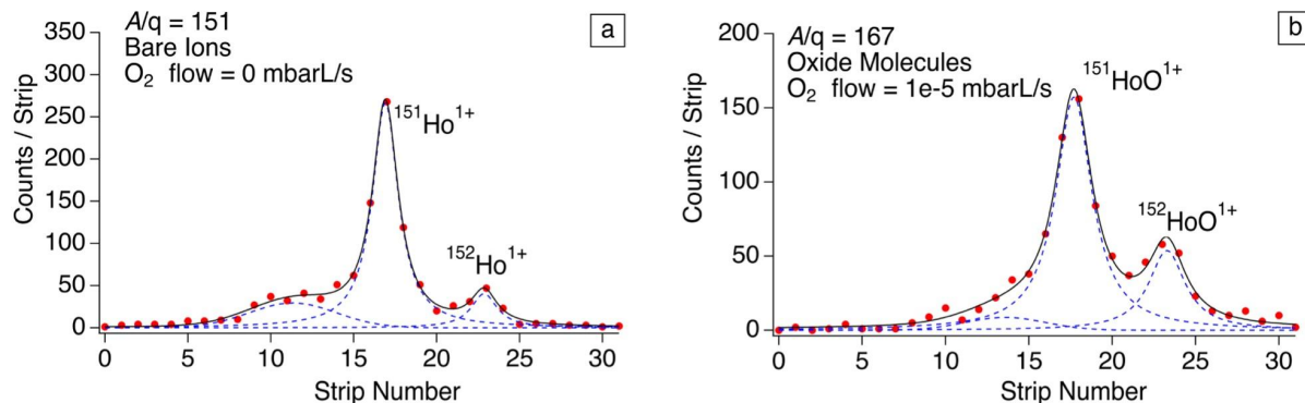
Figure 5.1: LBNL Data taken at the FIONA focal plane, where ions of holmium isotopes were reacted with oxygen ( \text{O}_2 ) gas to produce holmium-oxide molecules. The production of each was confirmed with mass-to-charge-ratio measurements. (a) Observed counts of ^{151-152}\text{Ho}^{1+} in the absence of \text{O}_2 gas. (b) The counts of oxide molecules ^{151-152}\text{HoO}^{1+} produced when a flow rate of 1e-5 mbarL/s \text{O}_2 gas was added to the system. Figure adapted from data in [Kwa21].
