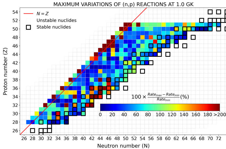
Figure 5: Maximum variation of the reaction rates for (n, p) reactions with isotopes relevant to the neutrino- p process when the JLM scaling parameters \lambda_x are varied within the estimated valid range.
