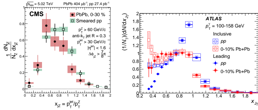
Figure 33: Example of measurements of jets balancing against a Z boson or a photon [592, 593].
