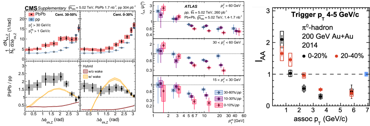
Figure 34: Example of measurements of hadrons produced in association with a Z boson (left, middle), or a \pi^0 .
