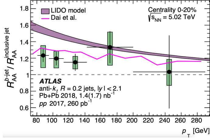
Figure 39: Ratio of b -jet R_{\text{AA}} to that of inclusive jets as a function of p_{\text{T}} in 0-20% Pb+Pb collisions at \sqrt{s_{\text{NN}}} = 5.02 TeV [816].
