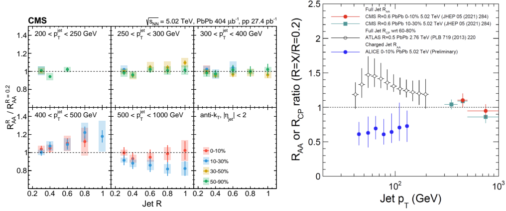
Figure 32: Jet R_{AA} measurements with large distance parameter as measured by CMS [586] (left) and ATLAS [645] compared to the machine learning extracted result from ALICE [737] (right).
