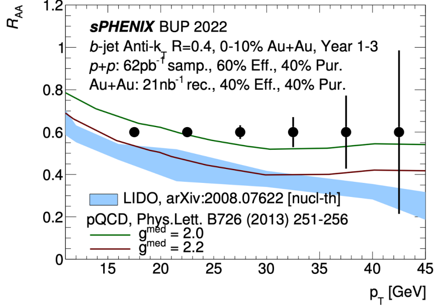
Figure 67: The anticipated statistical precision for measuring the R_{AA} of b -tagged jets compared to curves from a pQCD calculations with two coupling parameters to the QGP medium, g_{\text{med}} [1264], and a blue band representing a calculation based on the LIDO transport model [1271].
